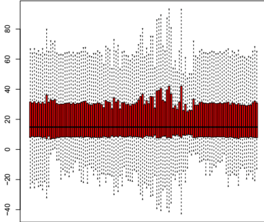
Supplementary Figure 2. Normalization of between arrays.
