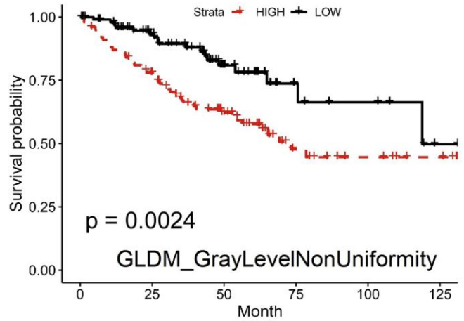
Supplementary Figure 1. Kaplan-Meier curves of groups with high-value and low-value “sphericity”, “surface-to-volume ratio”, “GLCM_correlation” and “GLDM_gray-level non-uniformity”.
