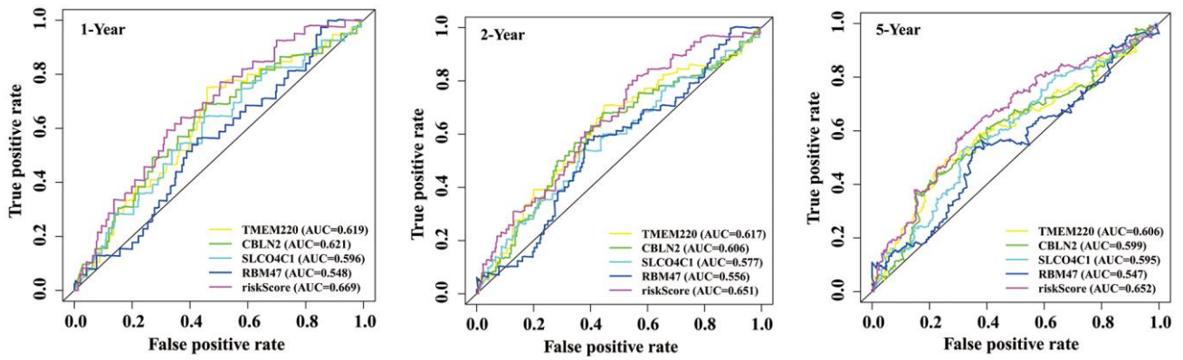
Supplementary Figure 1. Comparison of prognostic accuracy between 4 gene signature and single mRNAs.
